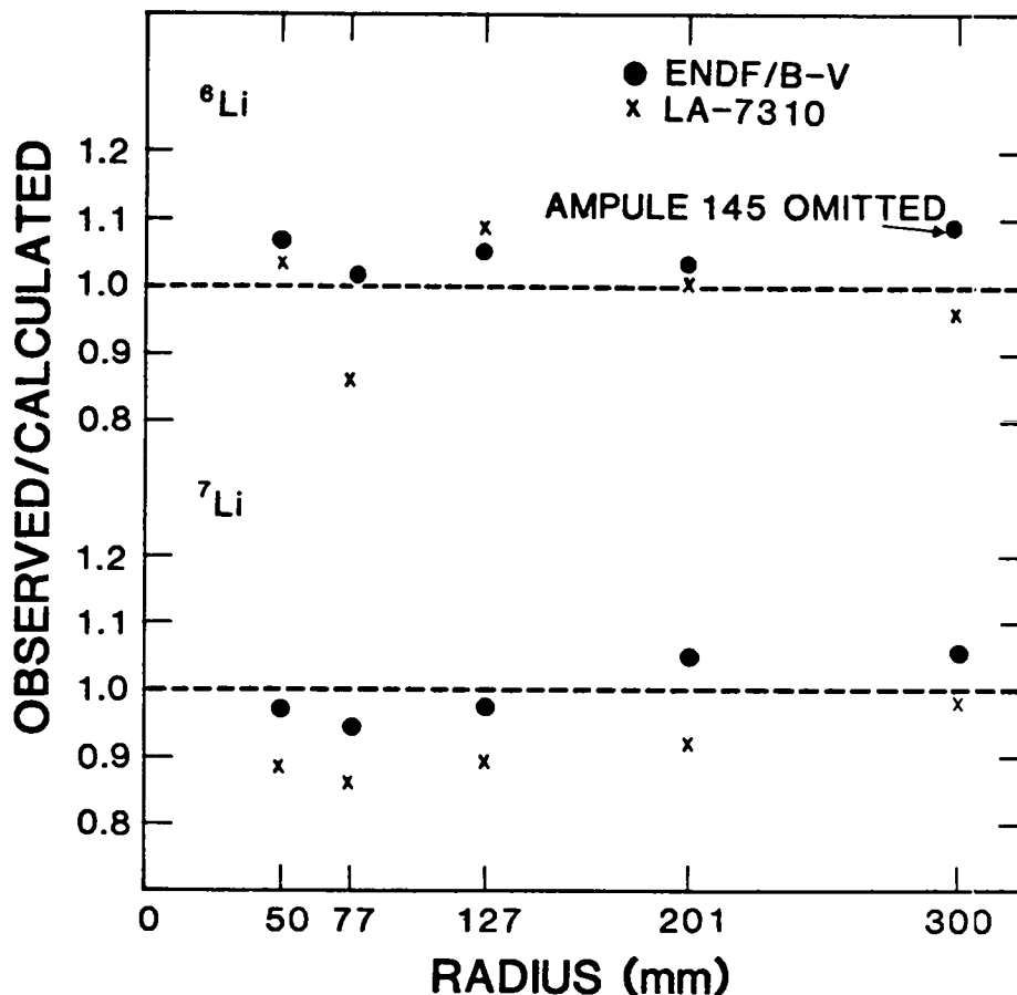
Fig. 4. Average observed-to-calculated tritium production at each radius. The present work is based on ENDF/B-V cross sections for transport and production. The LA-7310 values were taken from calculation IV of Tables VI and VII in Part II of that document.
